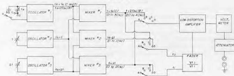
Figure 2. Functional block diagram illustrating the method of generating two-frequency signals.
